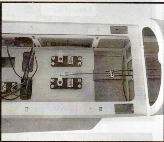
RUDDER PUSHROD HORN INSTALLATION.
